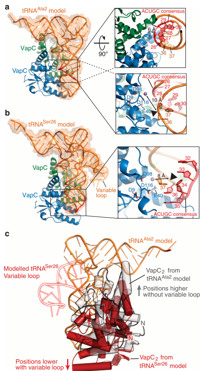
Figure 8 | VapC-mt4-tRNA docking simulations. (a) Predicted binding of a (VapC-mt4) 2 (blue and green) to tRNA Ala2 (Type I tRNA homologue, tRNA Phe model shown in orange; PDB accession code 4TNA) using a protein-RNA docking simulation programme 3dRPC. The consensus sequence 5'-ACUGC-3' is highlighted in red and boxed. The upper right boxed magnification shows a 90° rotated view highlighting the proximity of the tRNA consensus sequence to the VapC monomer not thought to be involved in activity (green). The lower right boxed magnification is a detailed view of the cleavage site. The VapC-mt4 key residues, tRNA consensus sequence and the target nucleotides are shown as sticks, with a black triangle indicating the cleavage site. (b) Predicted binding of a (VapC-mt4) 2 (blue and green) to tRNA Ser24/Ser26 (Type II tRNA homologue, tRNA Leu model shown in orange; PDB accession code 3UZ3). The expanded variable loop of tRNA Ser26 is depicted in orange outline and the consensus sequence 5'-ACUGC-3' is highlighted in red. The boxed magnification is a detailed view of the cleavage site showing the VapC-mt4 key residues, the tRNA Leu consensus sequence and the target nucleotides are shown in sticks, with a black triangle indicating the cleavage site. The extrapolated position of a divalent cation is shown as a purple sphere in both a,b. (c) A comparison of (VapC-mt4) 2 binding, highlighting the positional shift in tRNA binding depending on the target tRNA type (grey, tRNA Ala2 ; red, tRNA Ser24/Ser26 ). The presence of expanded variable loop in tRNA Ser26 (shown in red outline) influences the binding of VapC-mt4 (positions lower in anticodon loop) possibly explaining the difference observed in target cleavage sites. Convention when numbering tRNA bases dictates that the anticodon bases are numbered 34–36. This convention is followed in a–c. Note however that in the case of tRNA Ser26/Ser24 (b,c) the actual base numbers for the anticodon are 35–37.
